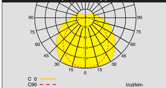
Luminous intensity distribution curve d 2GD E 2... (twin lamp)
